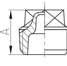
Solid Plug
