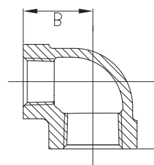
90° Reducing Elbow
