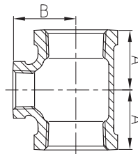
Reducing Tee
