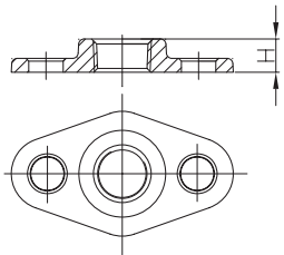
Wastenut
