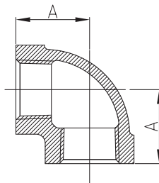
90° Reducing Elbow
