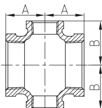
Reducing Cross
